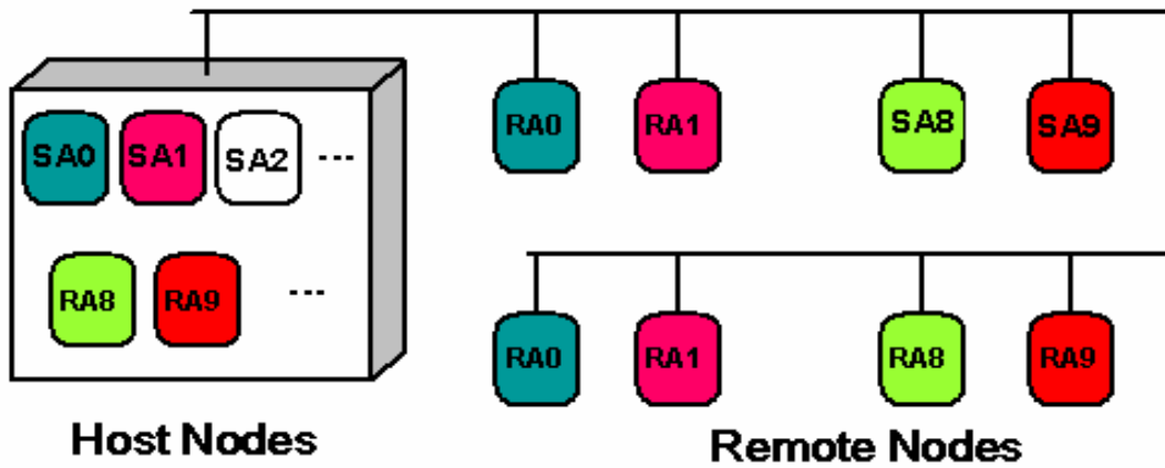
Figure 1.2 FRnet structure
